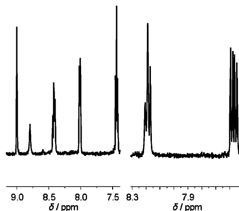
Figure 1. Expansion of regions of the 500 MHz 1 H NMR spectra of the polycycles 9a (left) and 10a (right). For polycycle 9a , signals for two rotamers are present, whereas for 10a , the sides of the p -cyanophenyl ring are diastereotopic. On the NMR timescale, rotation about the single bond between the sp 3 -hybridised bridgehead carbon and the substituted phenyl ring is slow.
