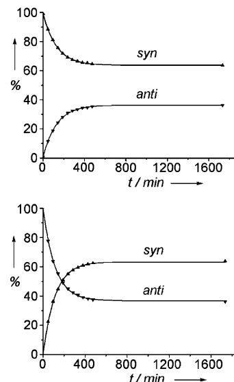
Figure 3. Equilibration of the syn (top) and anti (bottom) rotamers of polycycle 9a at 288 K in acetonitrile/water.
