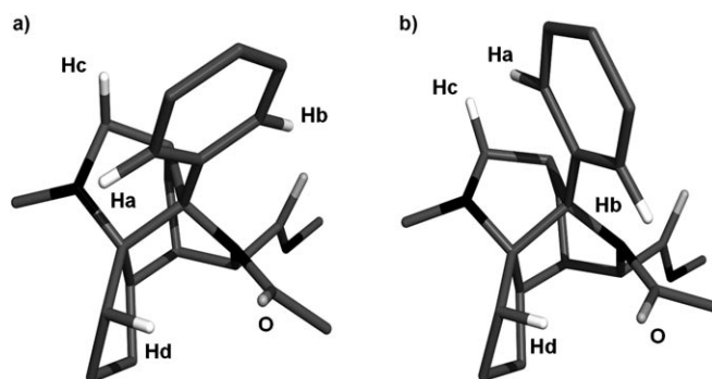
Figure 4. Minimised structure (a) and TS structure (b) for polycycle 13b . An animation for the bond-rotation process is provided in the Supporting Information.
