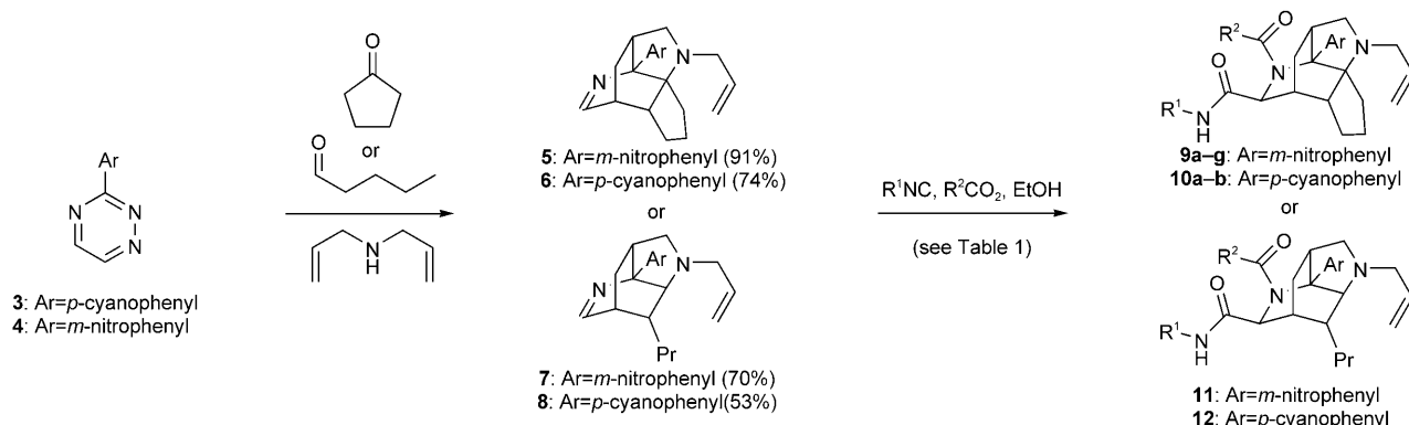
Scheme 1. Preparation of polycyclic compounds 9–12 .
