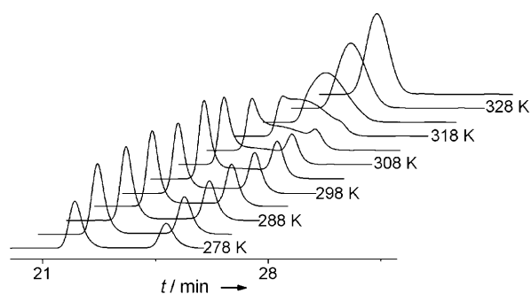
Figure 2. Chromatograms for polycycle 9a determined by using variable-temperature analytical HPLC in acetonitrile/water.
