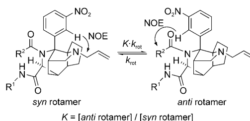
Scheme 2. Interconversion of the syn and anti rotamers of polycyclic compounds 9 and 11 . The configurations of the rotamers of 9g were determined through observation of diagnostic NOE interactions.
